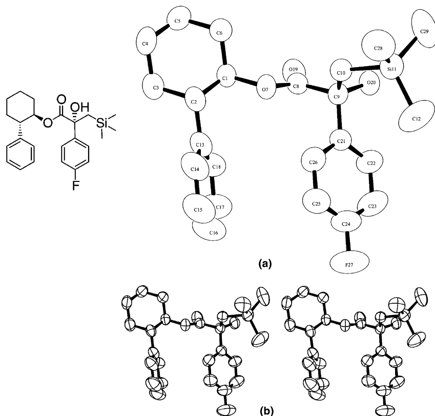
Figure 1. (a) Molecular structure of 10 (–) with atomic numbering and (b) stereoscopic view of 10 (–).
