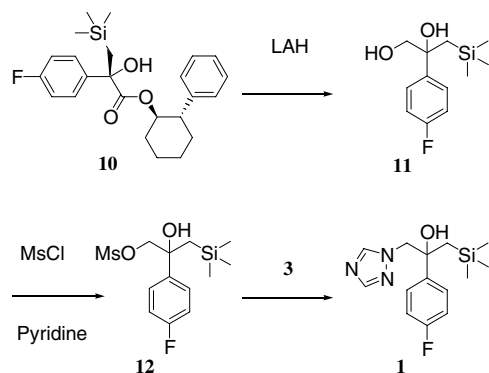
Scheme 3. Novel method for the preparation of 1 .
