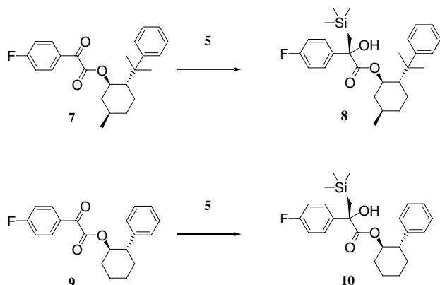
Scheme 2. The Grignard reaction of 5 with phenylglyoxylates.
