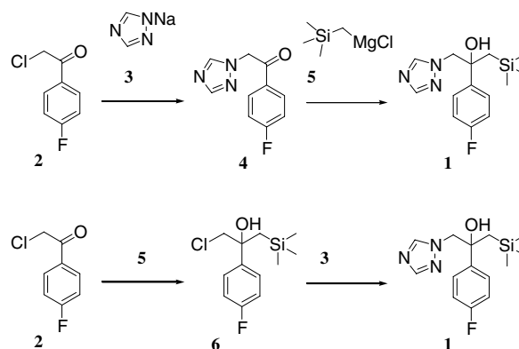
Scheme 1. Our previous method for the preparation of 1 .
