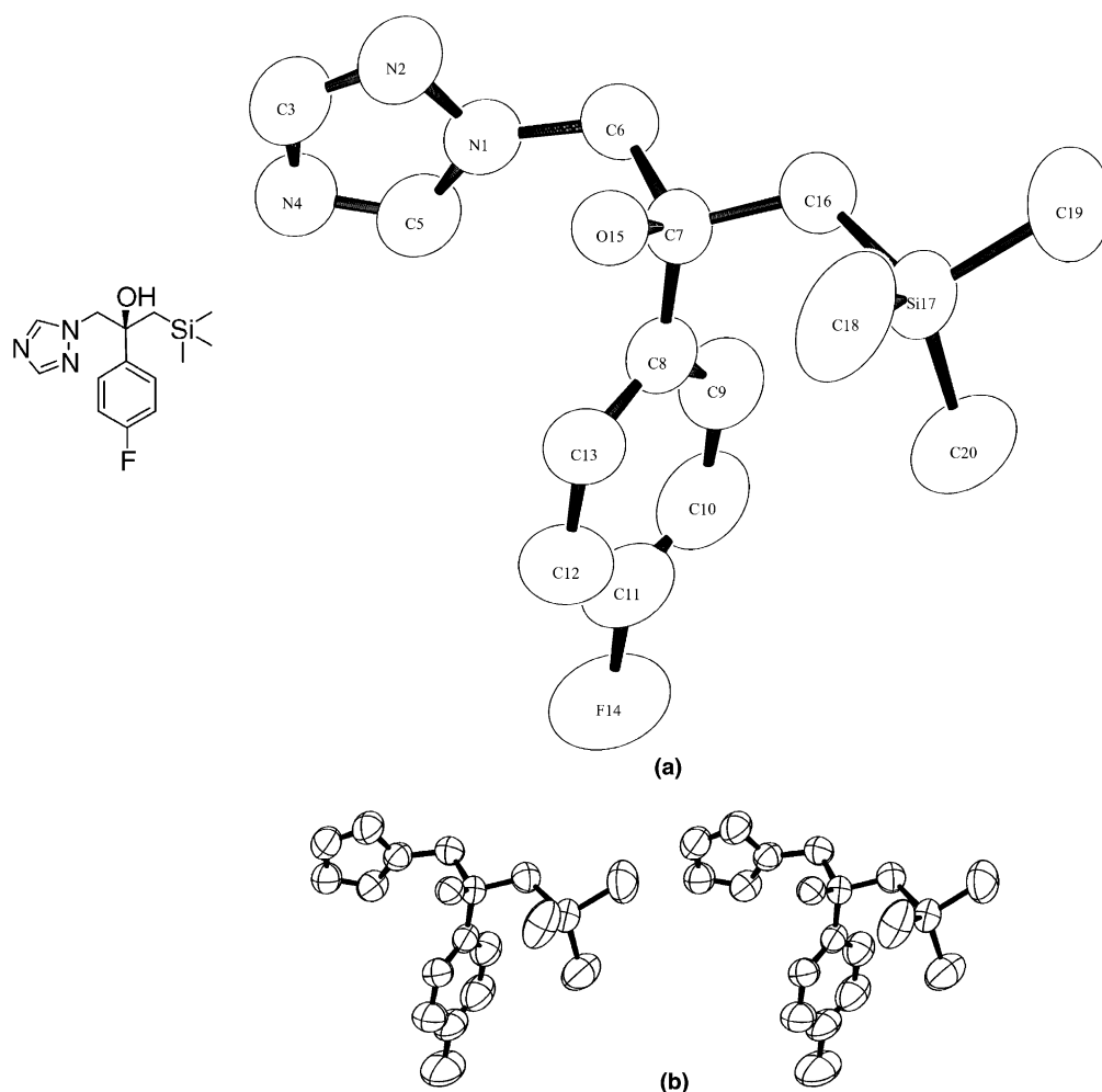
Figure 2. (a) Molecular structure of 1 (+) with atomic numbering and (b) stereoscopic view of 1 (+).
